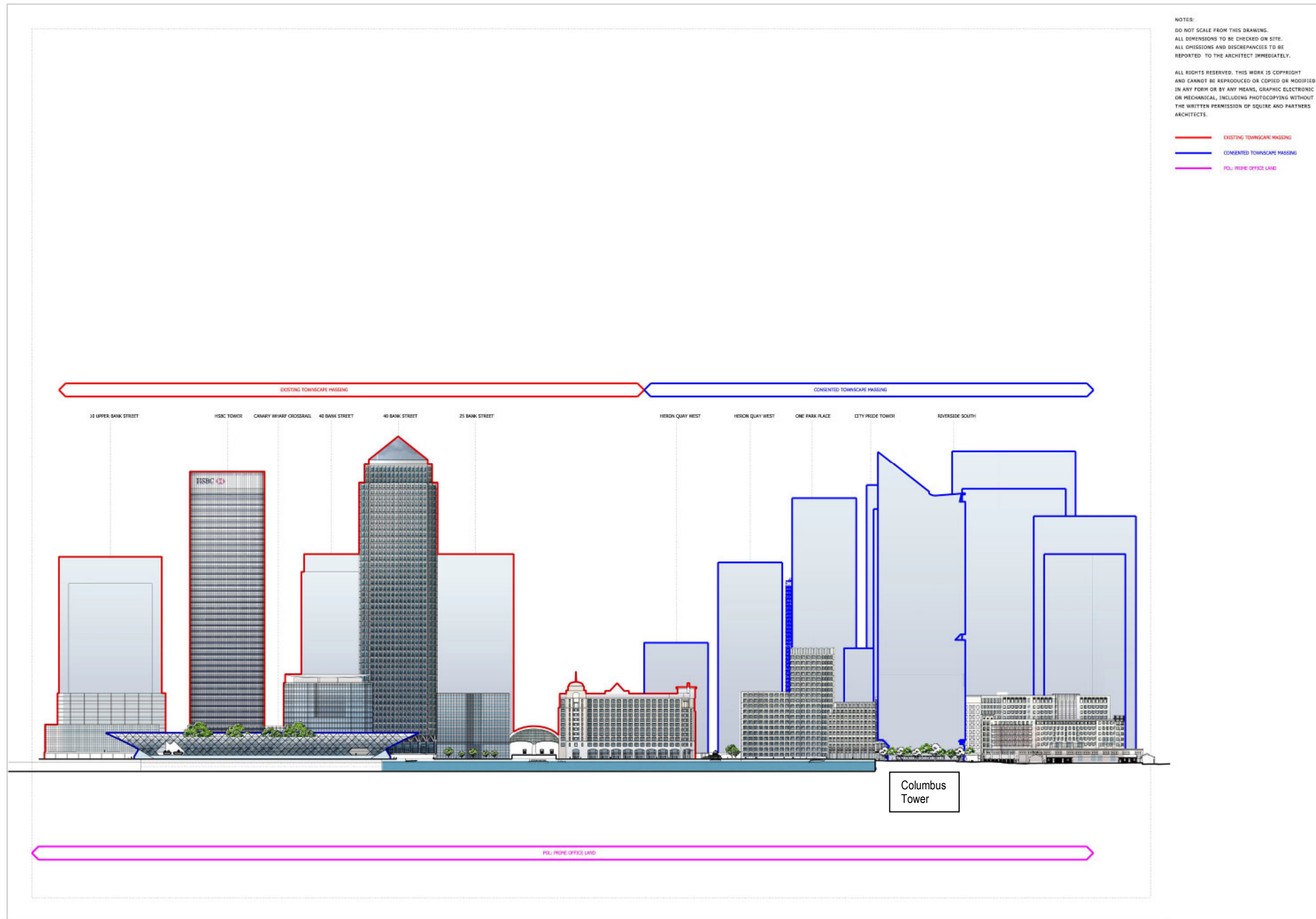
Figure C2: east-west section looking south towards Canary Wharf cluster, showing proposed Columbus Tower project (on right)
